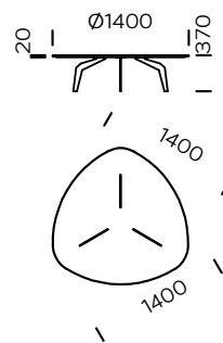
Triangular table FEZA 1400
