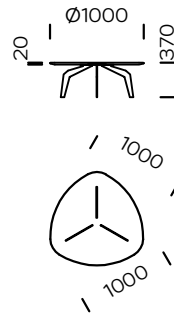
Triangular table FEZA 1000
